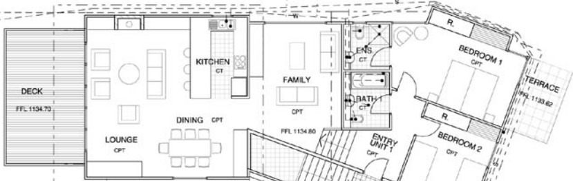
01 FIRST FLOOR PLAN SCALE 1/200
